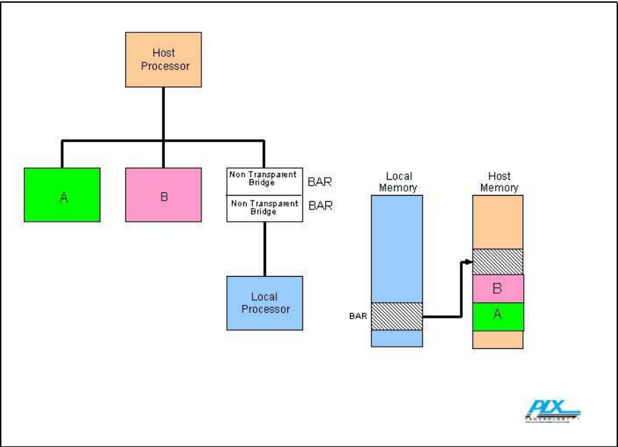
Figure 0-2: Direct Address Translation
