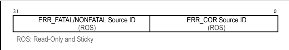
Figure 15-29: Advanced Source ID Register
