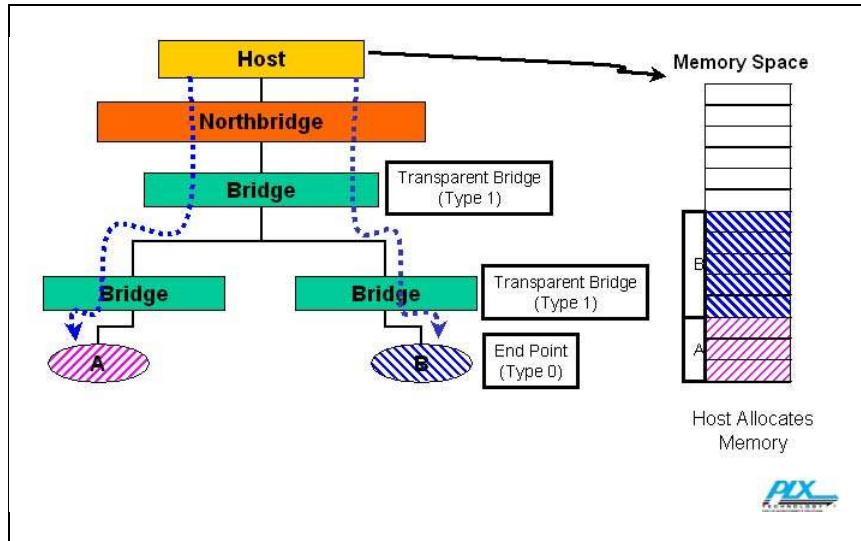
Figure 0-1: Enumeration Using Transparent Bridges
