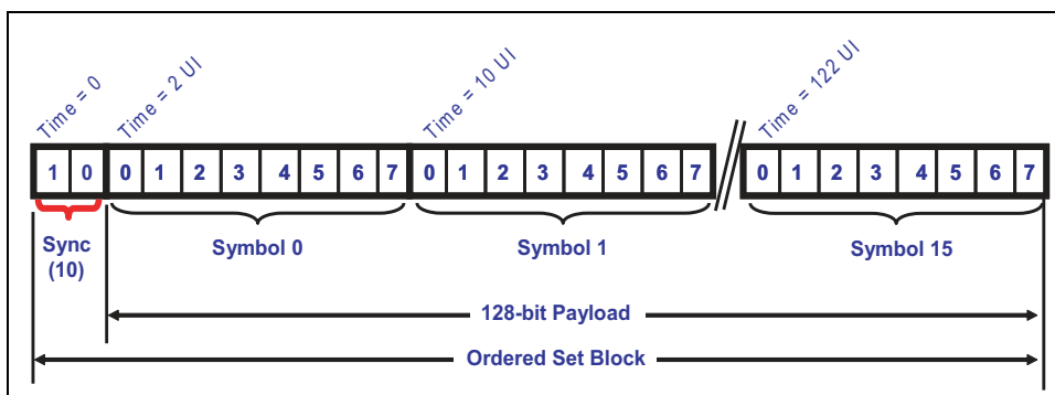
Figure 12-5: Gen3 x1 Ordered Set Block Example
