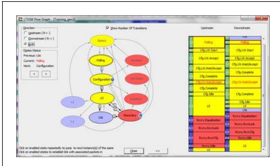
Figure A-10: LTSSM Graph Shows Link State Transitions Across the Trace
