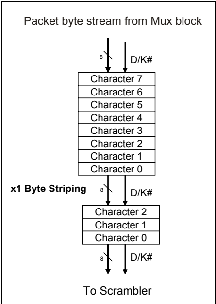
Figure 11-8: x1 Byte Striping
