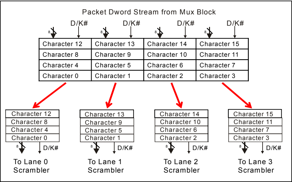
Figure 11-9: x4 Byte Striping
