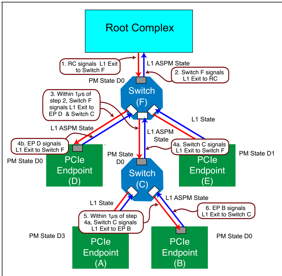
Figure 16-20: Switch Behavior When Upstream Component Signals L1 Exit
