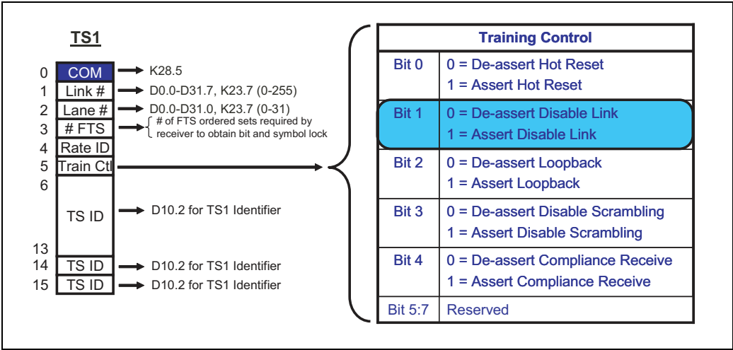
Figure 18-7: TS1 Ordered-Set Showing Disable Link Bit
