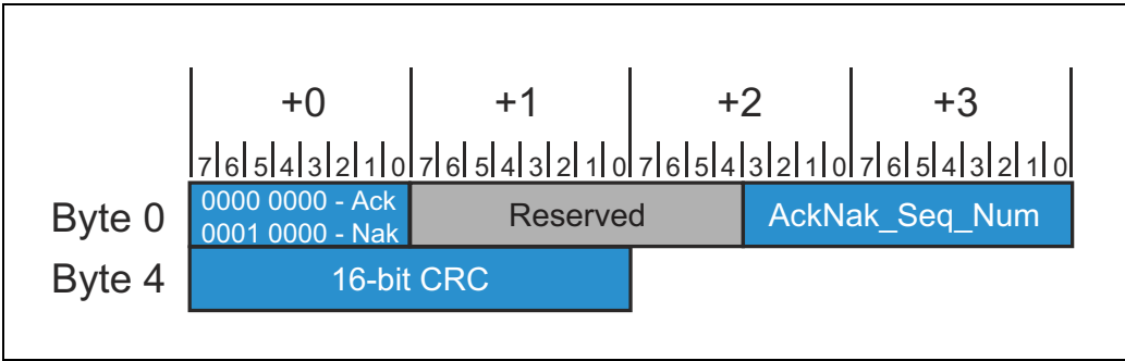
Figure 9-3: Ack Or Nak DLLP Format
