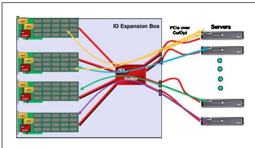
Figure 0-6: Server Failover in 1 + N Failover Scheme
